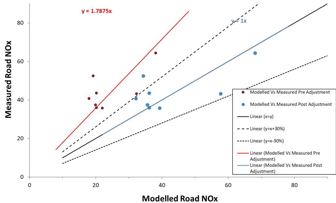
Figure D-0-6 Modelled road NOx vs measured road NOx
