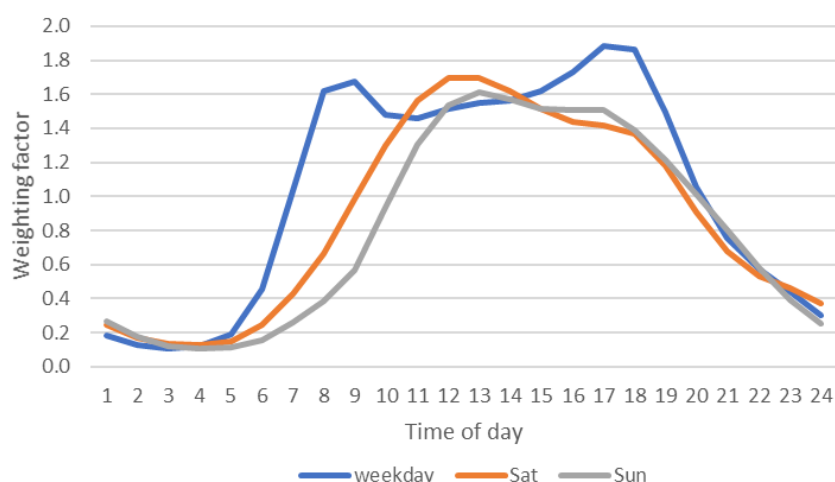
Figure D-0-5 Diurnal traffic movements used in the dispersion model study
