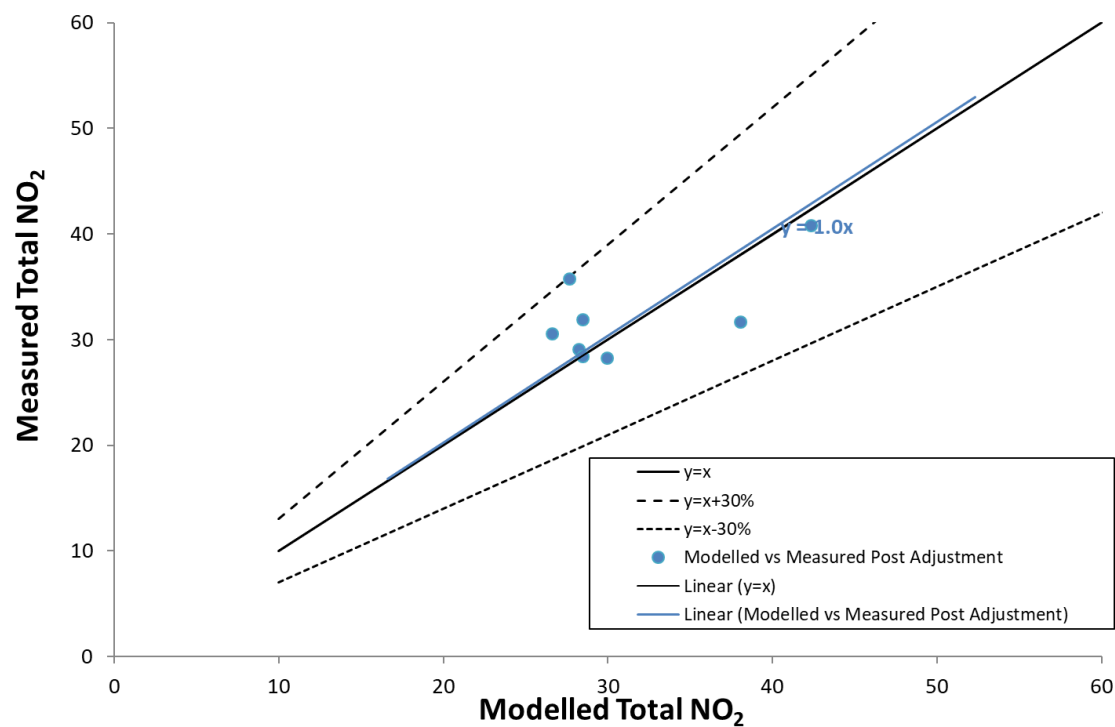
Figure D-0-7 Modelled total NO 2 vs measured total NO 2
